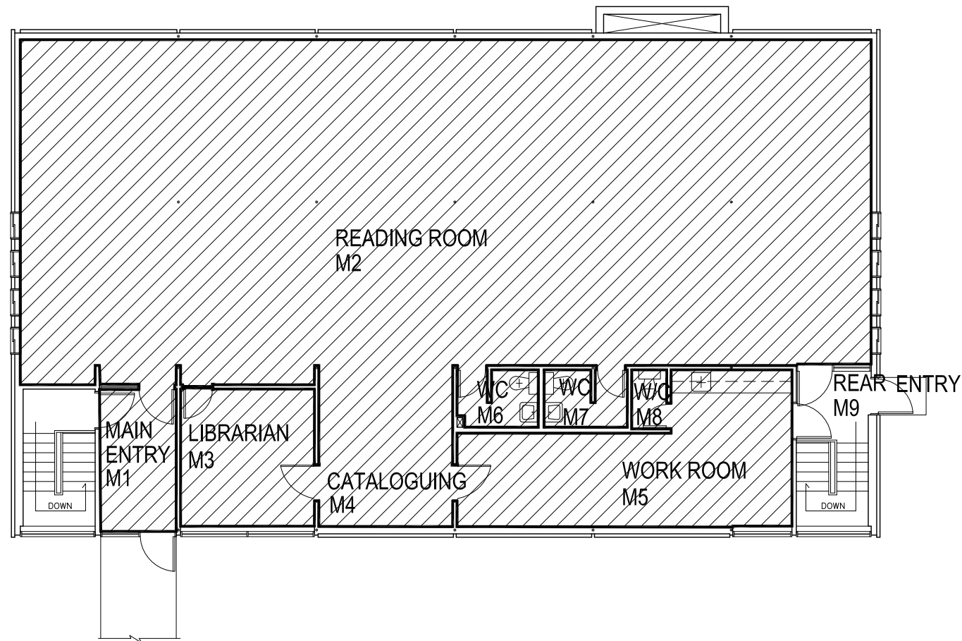
MAIN FLOOR PLAN 955 COTTONWOOD WINDSOR PARK LIBRARY
